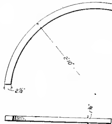
Figs. 1239-1240. Canopy Return-ribs.
